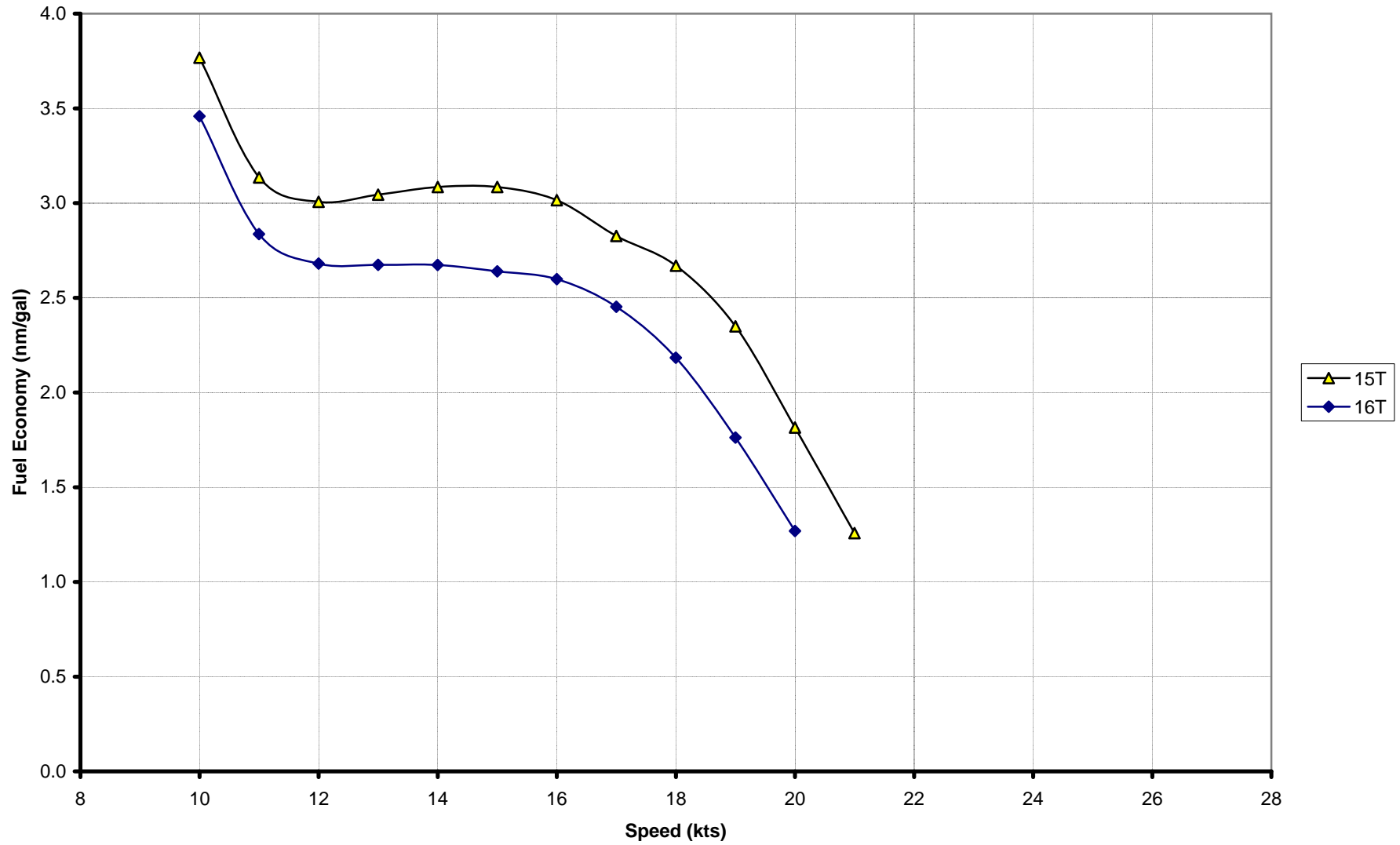
Fuel Economy v. Speed
